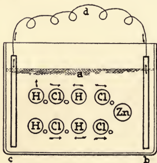
EXPLANATION OF A GALVANIC CELL
