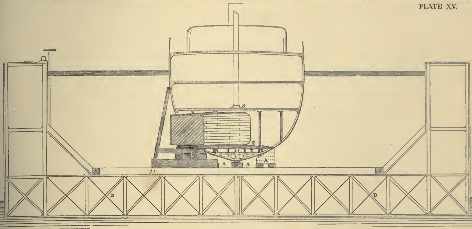
SECTION
