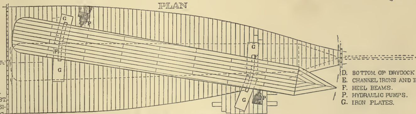
SLUNG OBELISK IN STEAMER'S HOLD EMBARCKING THE OBELISK
