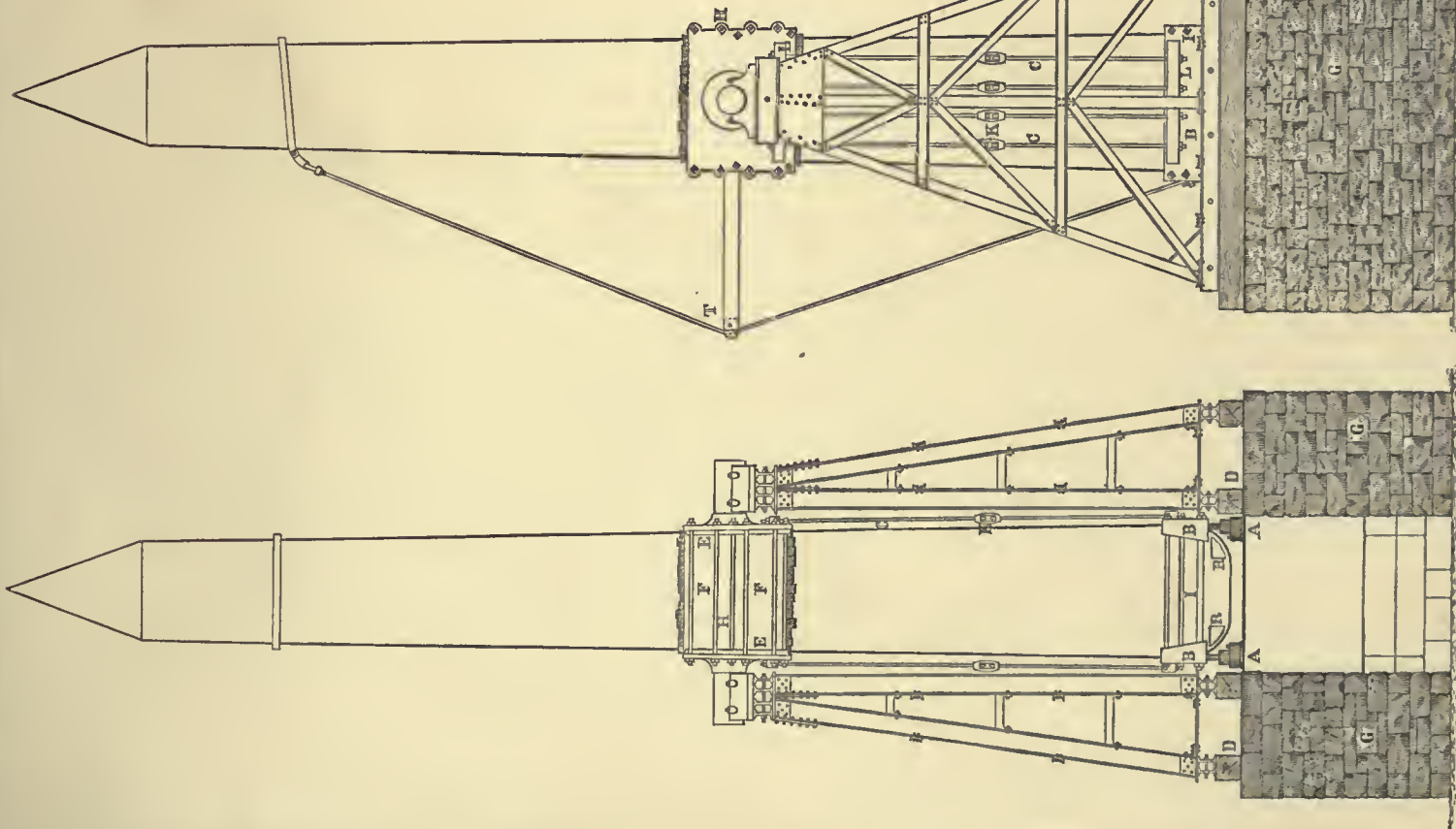
LOWERING ON THE PEDESTAL
