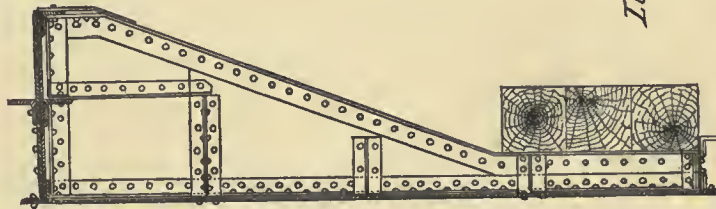
Sectional Plan through bearing showing wing.
