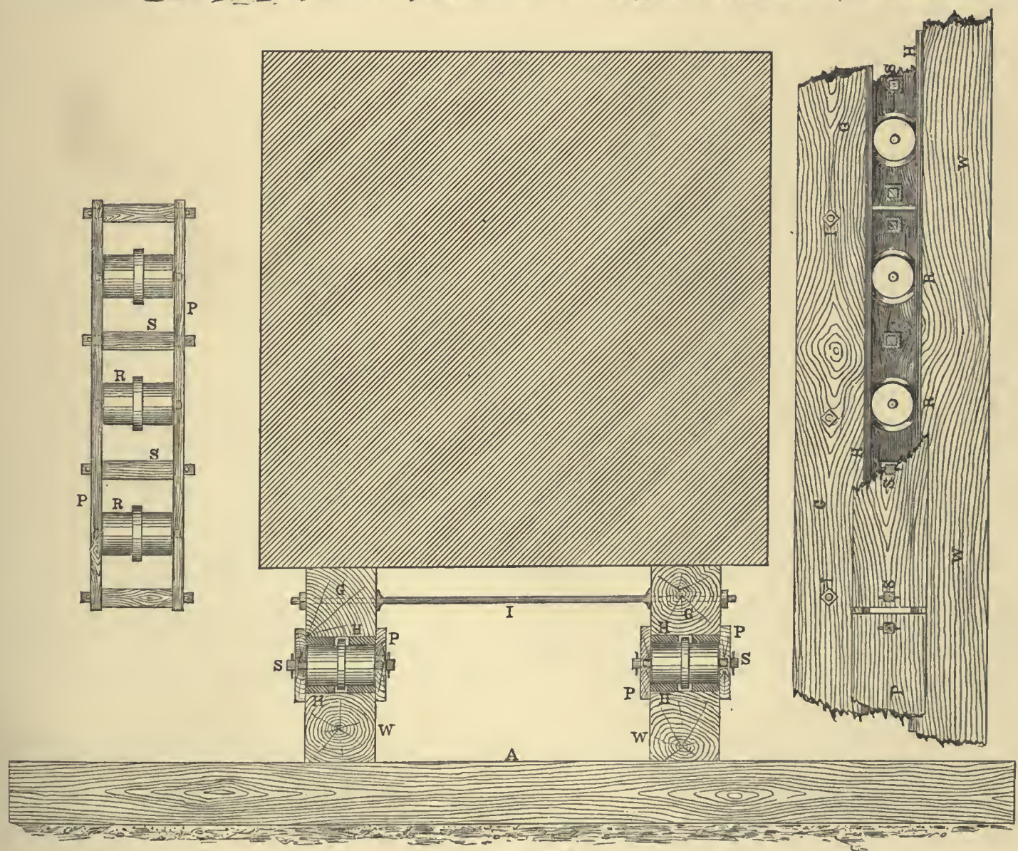
IRON CHANNELS AND MARINE RAILWAY
