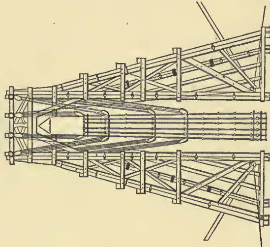
Perspective view of Structure.
