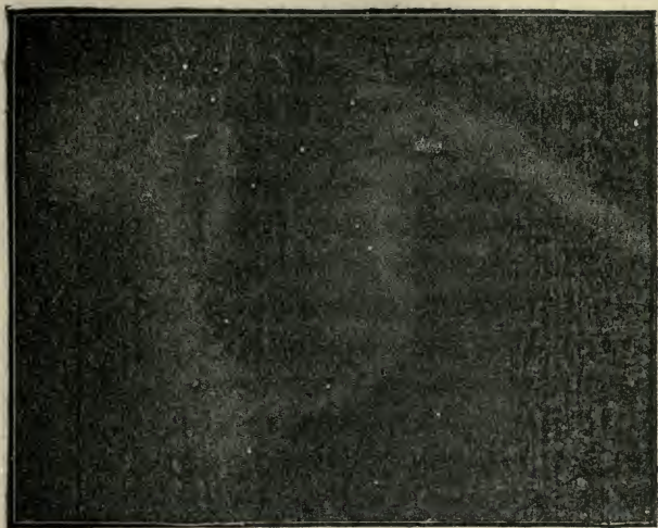
Fig. 9.—The Shield of Sobieski.
