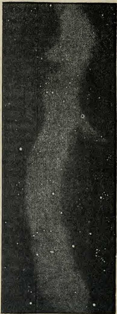
Fig. 10.—The Milky Way.
