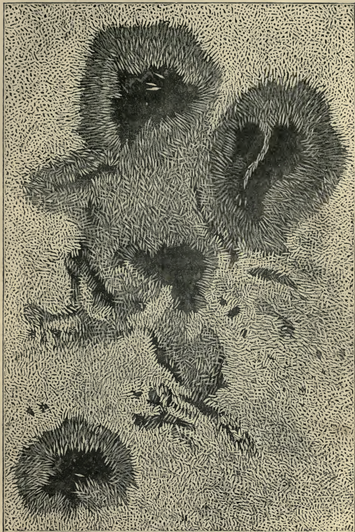
Fig. 2.—Group of Solar Spots observed in 1864 by Nasmyth.
