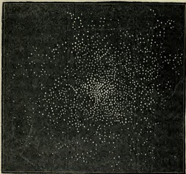
Fig. 8.—The Nebula of the Centaur.
