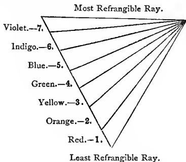
Fig. 33. PRISMATIC SPECTRUM.
