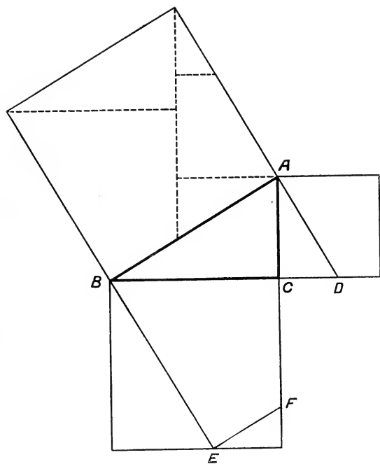
FIG. 3. Diagram to illustrate the Theorem of PYTHAGORAS.
